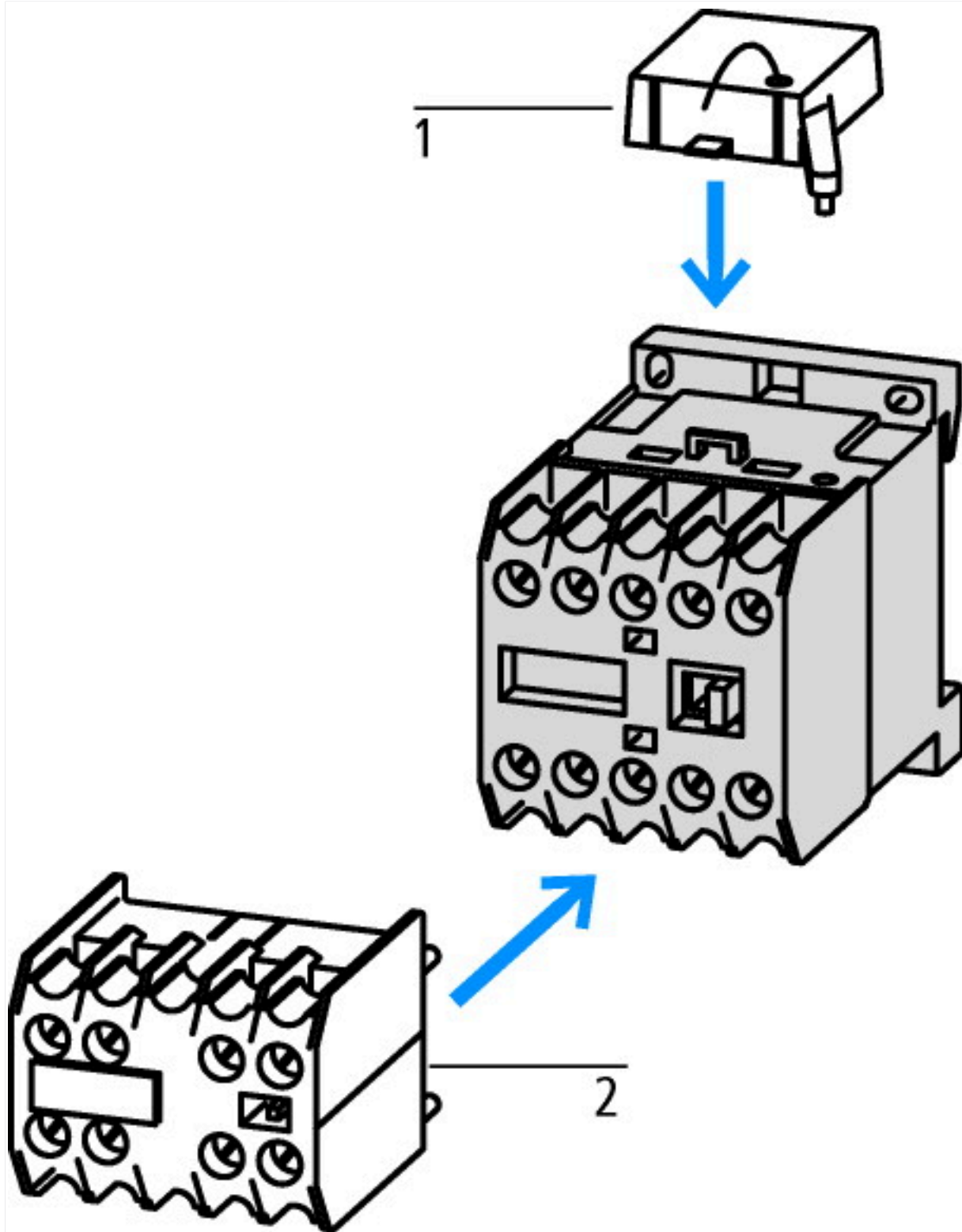
1: Suppressor 2: Auxiliary contact module
